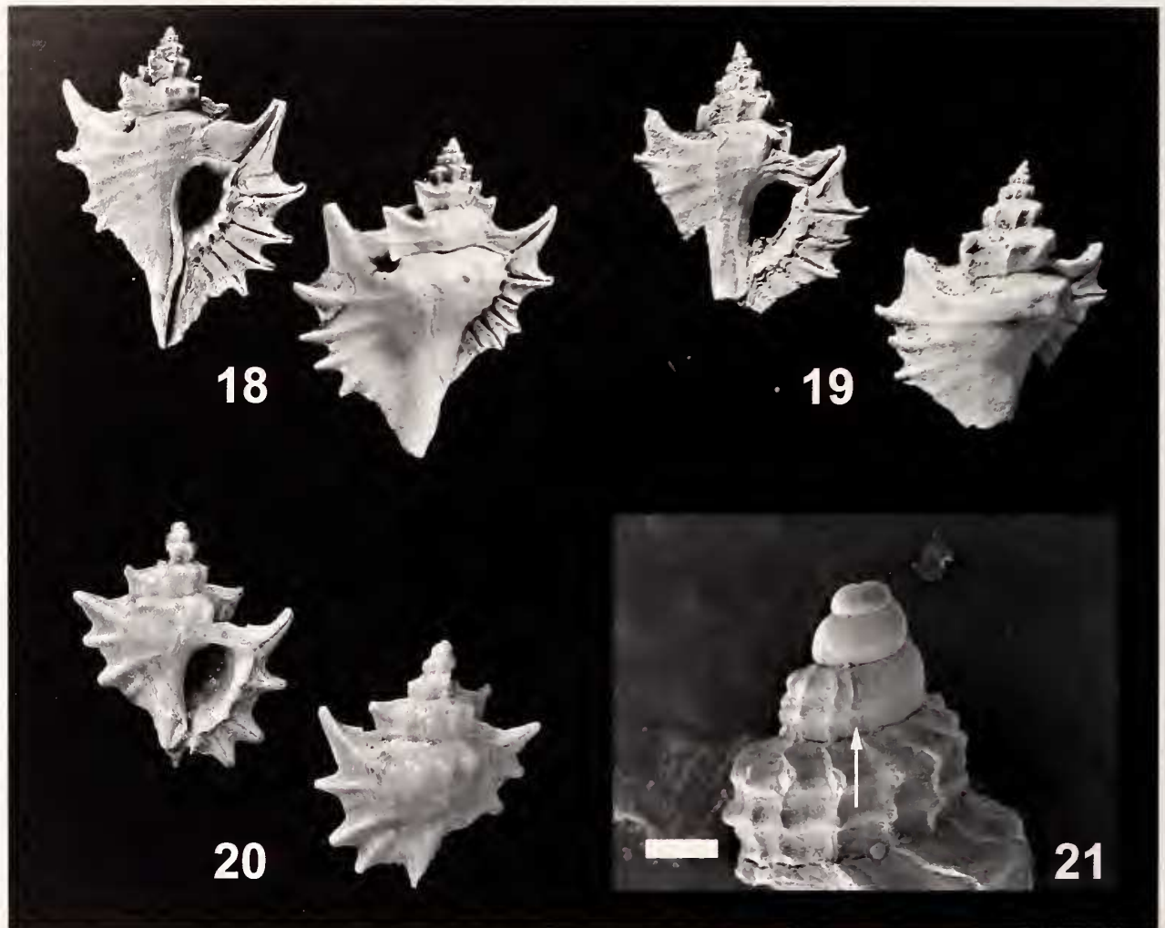
Figures 18–21. Eupleura lehneri Jung, 1969. Figure 18. USNM 645346 (Holotype); locality: Melajo River, northeastern Trinidad; Early Pliocene, Melajo Clay Member of Springvale Formation (= USGS 21178); height 27.0 mm, diameter 19.6 mm. Figure 19. USNM 519549 (Paratype); locality: Same as Fig. 18; height 20.3 mm, diameter 17.8 mm. Figure 20. NMB H 18316; locality: Quitarfa, Río Banano, Limón Province, Costa Rica; Early Pliocene, Río Banano Formation (= NMB 18096, PPP 00679); height 11.8 mm, diameter 10.2 mm. Figure 21. USNM 519550; locality: Same as Figure 18; scanning electron micrograph of protoconch and early teleoconch whorls (scale bar = 200 \mu m; arrow points to protoconch/teleoconch transition).
